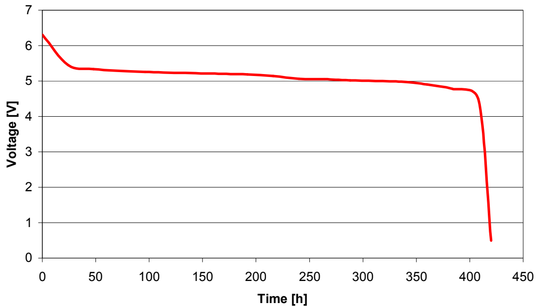
Discharge curve 82 ohm continous
