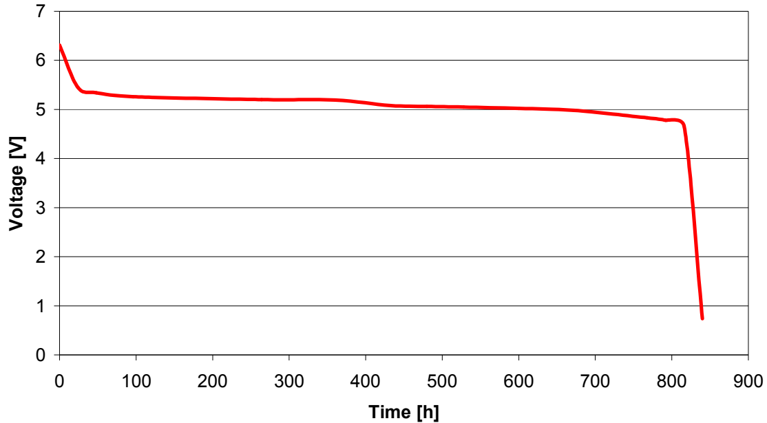
Discharge curve 82 ohm continous
