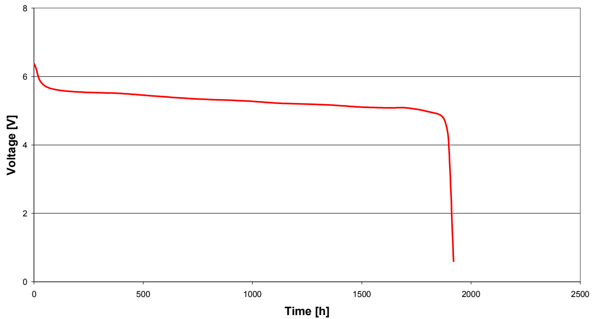
Discharge curve 164 ohm continuous
